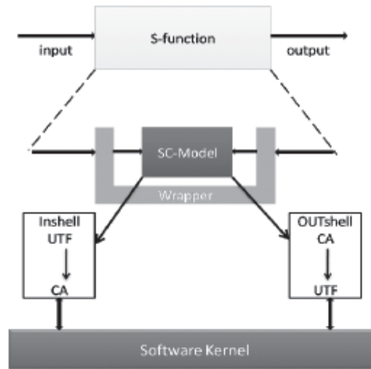
Figure 1. Using SystemC within Simulink S-Function
