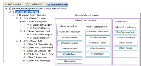
Figure 6: Concrete User Interface.
