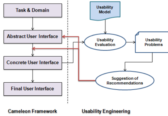
Figure 1: The proposed Usability Measurement Method.
