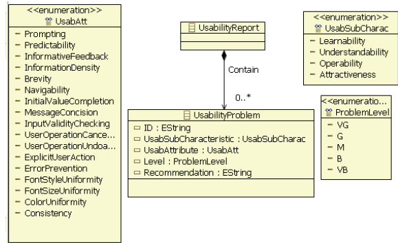
Figure 4: Usability Report Meta-Model.
