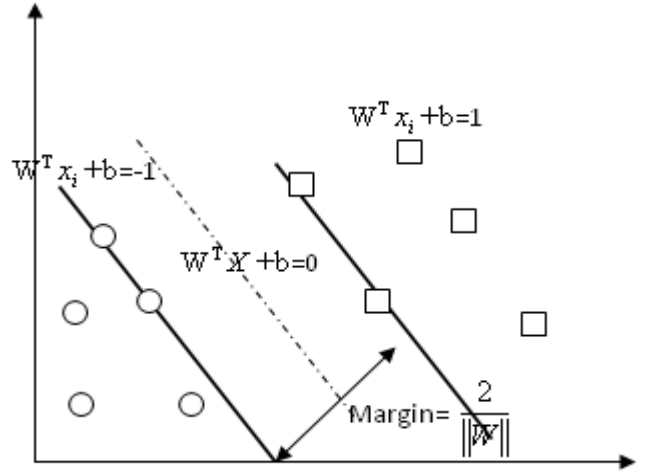
Figure 2. Separating hyper-plane between two classes
