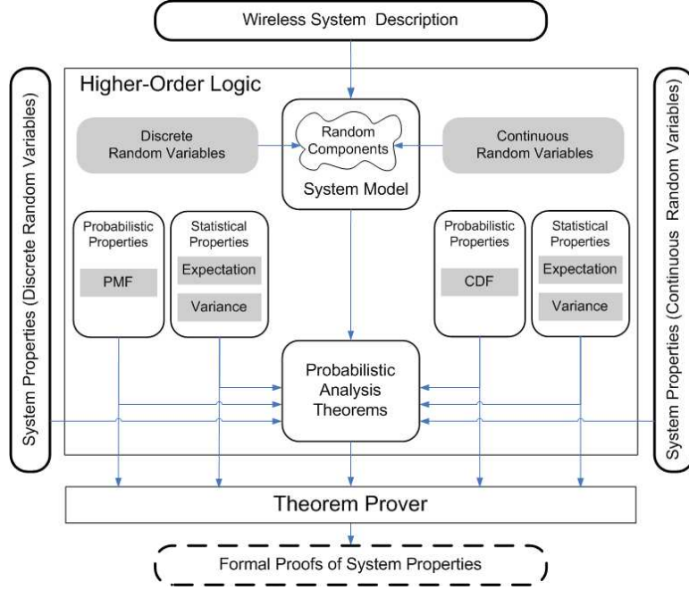
Figure 1: Theorem Proving based Probabilistic Analysis Framework for Wireless Systems.
