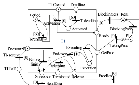
Figure 1. Task modeling with PTPN
